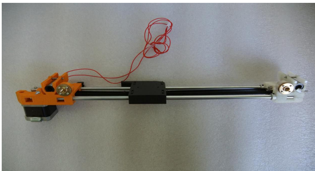
Figure 15 Q Assembly
